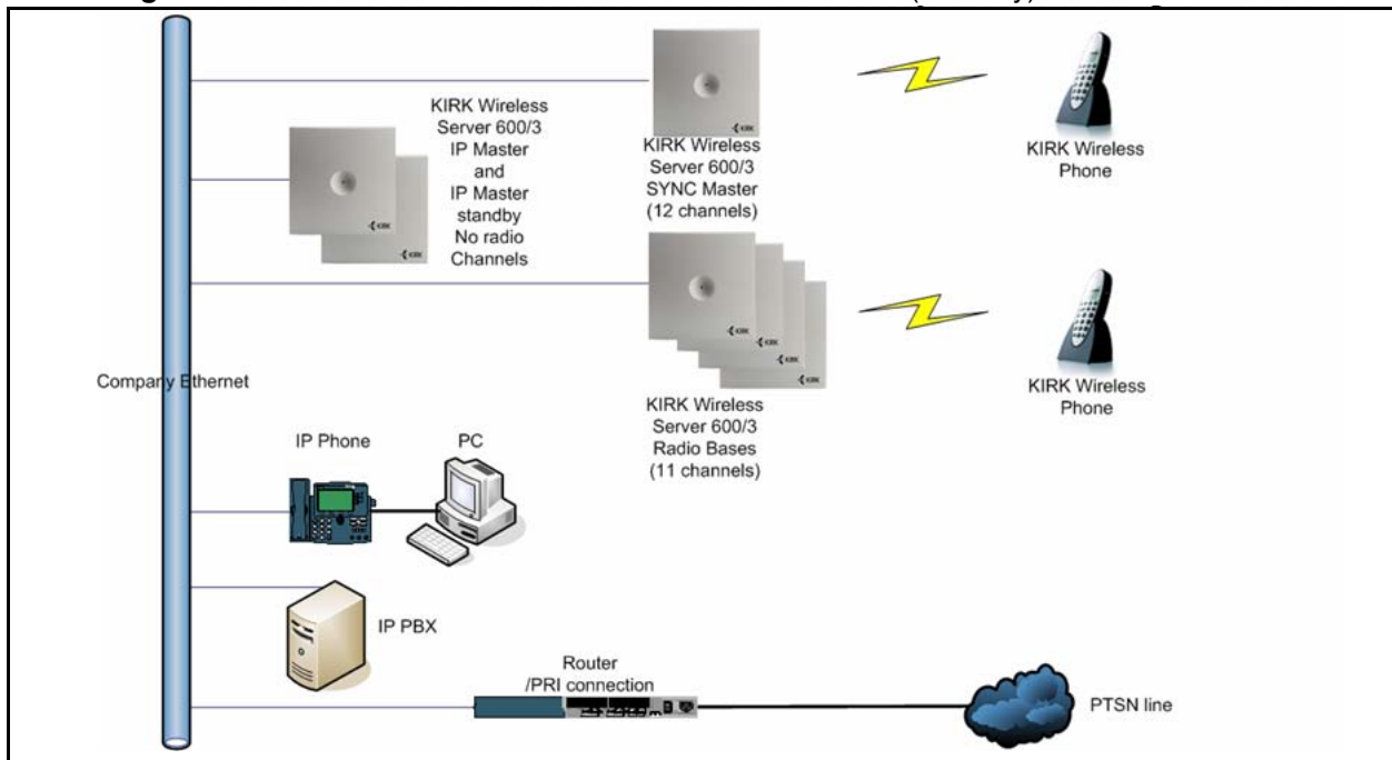
Figure 87 KWS600v3 Multi-cell installation with Alternative (Standby) Master
